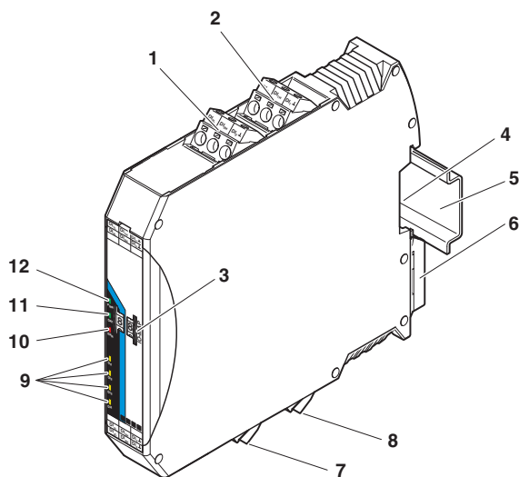
Figure 1 Function elements
