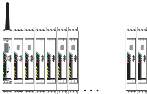
Figure 5 SATEL-LP connection station with up to 32 I/O extension modules
